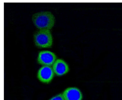
Fig. 2. ICC staining RPS3 in N2A cells (green). The nuclear counter stain is DAPI (blue). Cells were fixed in paraformaldehyde, permeabilised with 0.25% Triton X-100/PBS.
